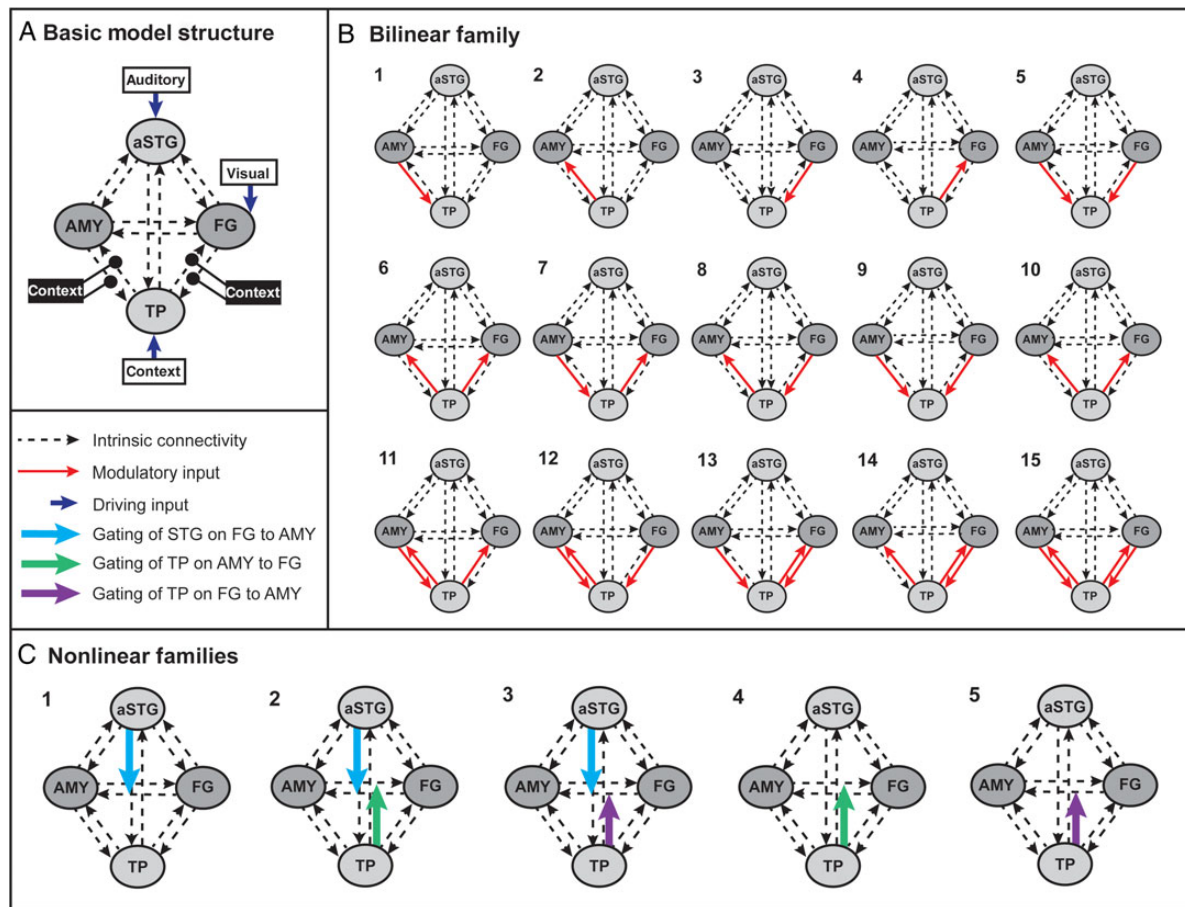
Figure 4. Model space. (A) Basic model structure with nodes, intrinsic connections (dash dotted arrows), and driving input (dark blue arrows). The “visual” driving input on FG includes all conditions containing a film clip (Fig. 1B1–6). The “auditory” driving input includes all conditions containing music (Fig. 1B4–7). The “context” driving input includes all conditions containing context (Fig. 1B2, 3, 5, and 6). For clarity, the modulatory input is labeled “context,” which in fact contains the 4 distinct modulatory inputs (neutral/sad context followed by a silent film clip or a film clip accompanied by music). (B) Bilinear model family with all possible bilinear modulations on TP–FG and TP–AMY coupling in both directions. (C) Nonlinear families; the bilinear model family was tested in all of the nonlinear families resulting in 90 models per subject.
